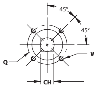
BottomView ISO5211
