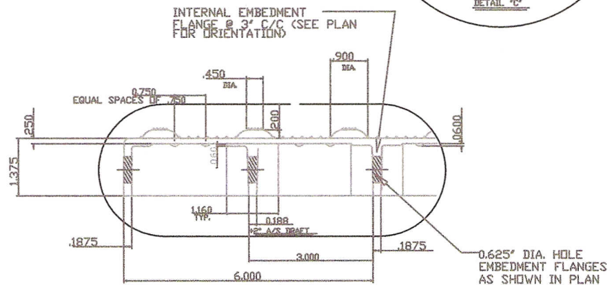
DETAIL "B"
