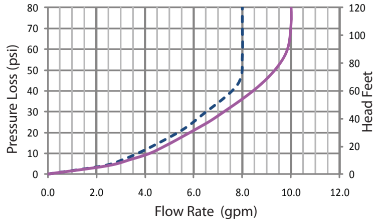
Pressure Loss
