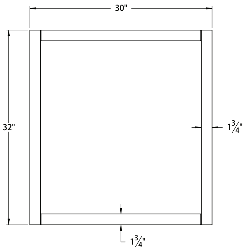
FRONT VIEW
