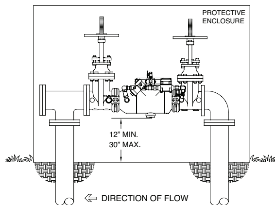
ZURN WILKINS MODEL 350ASTDA OUTDOOR HORIZONTAL INSTALLATION
