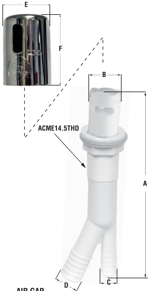
AIR GAP
