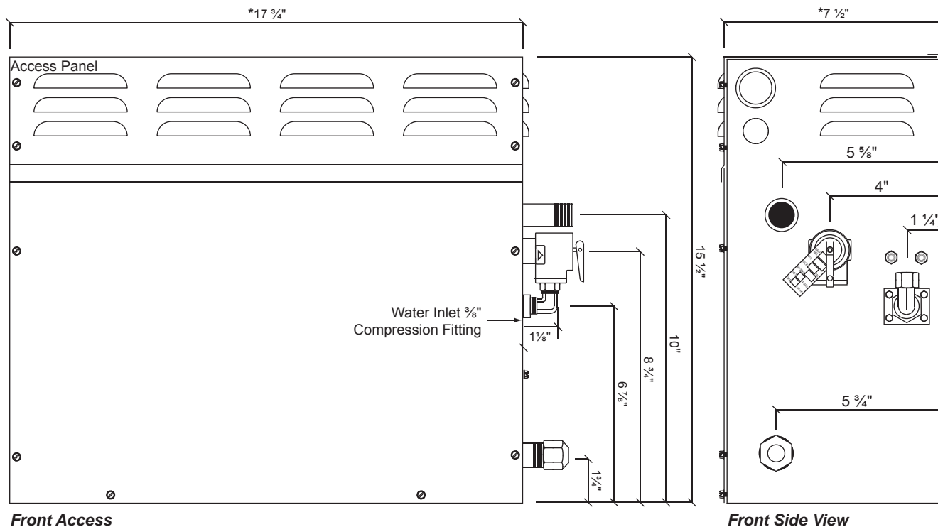
Front Access
