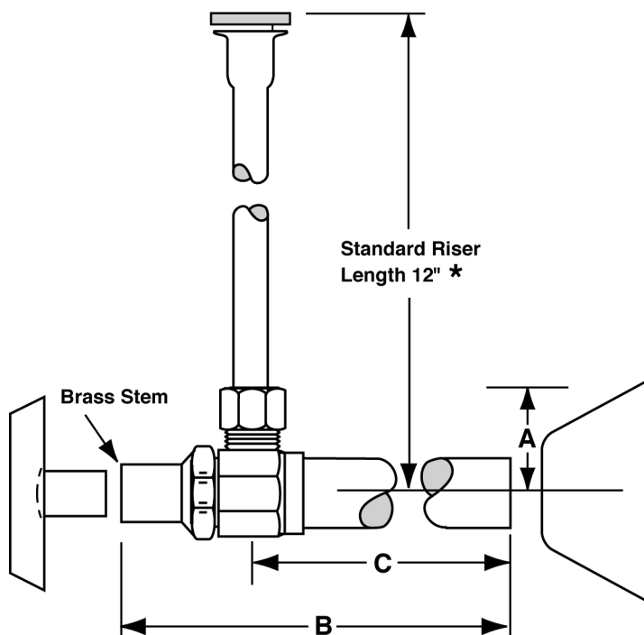
Loose Key with 5" Extension Tube
