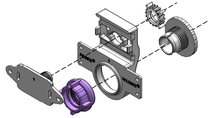
PEXRITE #731 "Exploded"
