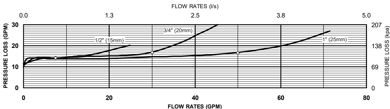
Capacity thru Schedule 40 Pipe
