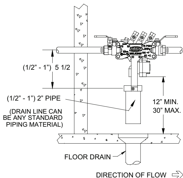
INDOOR INSTALLATION
