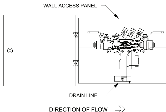
OUTDOOR INSTALLATION
