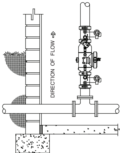
ZURN WILKINS MODEL 350ASTDABG INDOOR VERTICAL INSTALLATION
