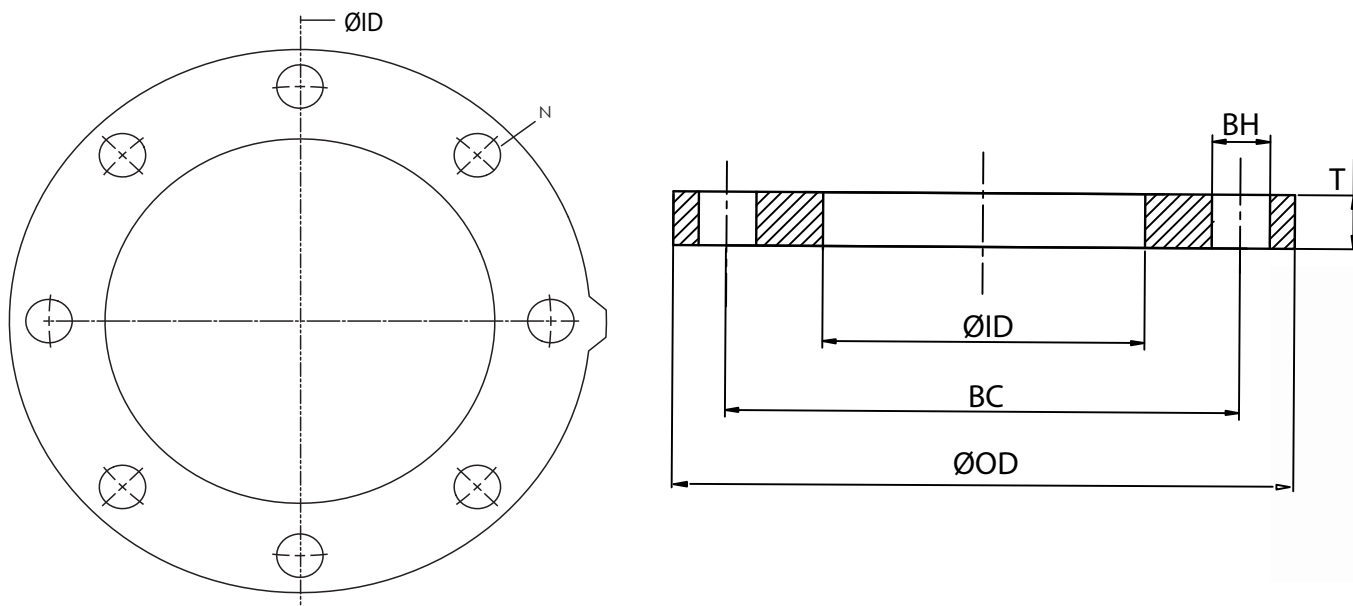
Dimensions (inches)
