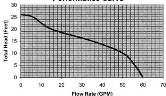
Performance Curve
