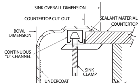
Installation Detail
